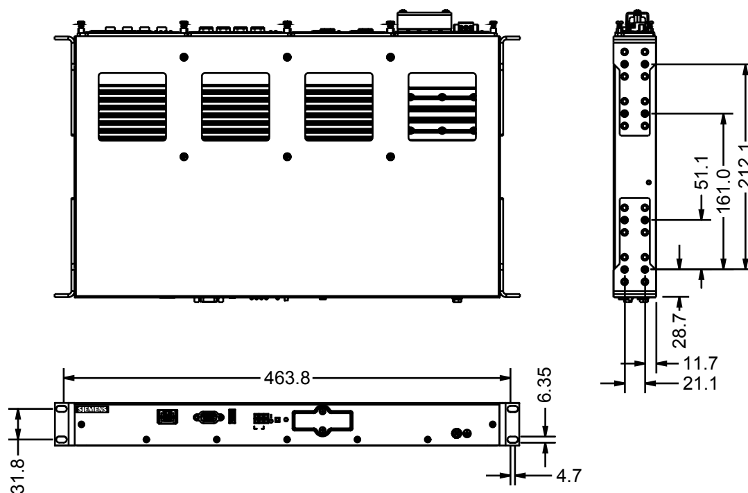
Figure 54: Rack Mount Dimensions
