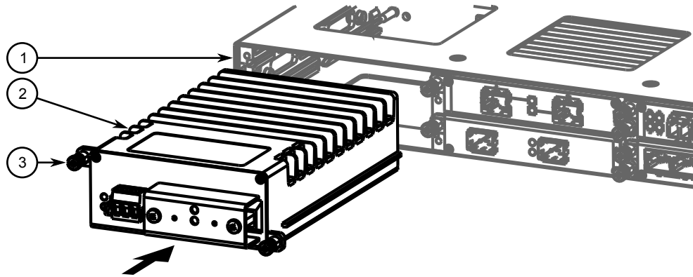
Figure 6: Installing a Power Supply
