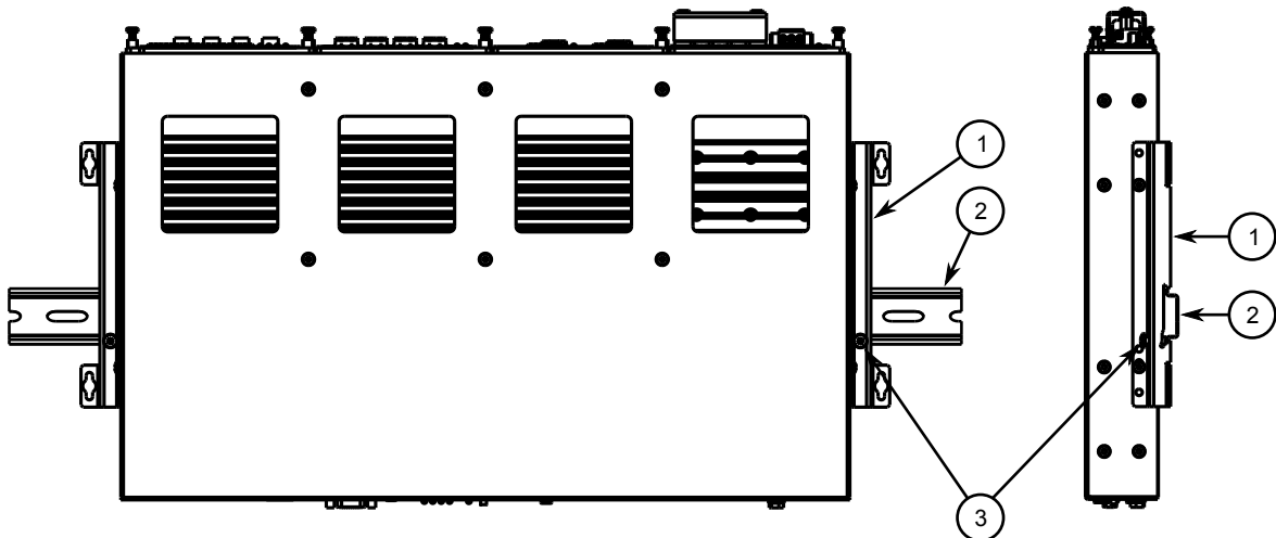
Figure 3: DIN Rail Mounting
