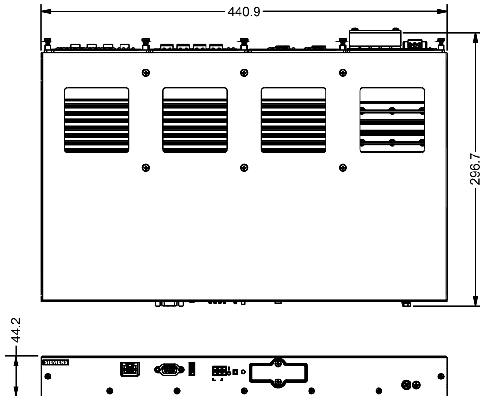
Figure 53: Overall Dimensions
