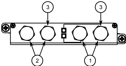
Figure 44: W12, W22 and W32 Cellular Modems 1. Main Antenna SMA Connector 2. Receive Diversity Antenna SMA Connector 3. Antenna for First/Primary Cell Modem
