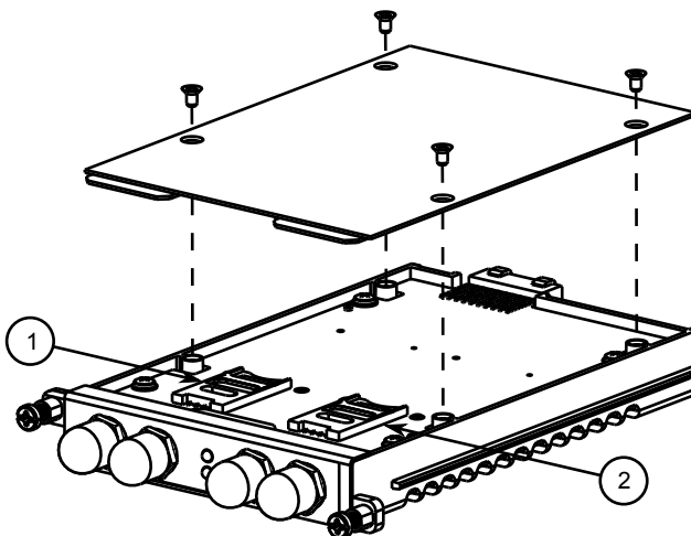
Figure 46: W12, W22, W32 Cellular Modem
