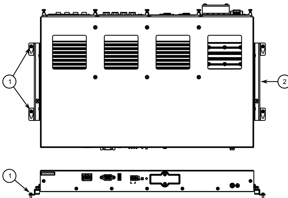
Figure 4: Panel Mounting
