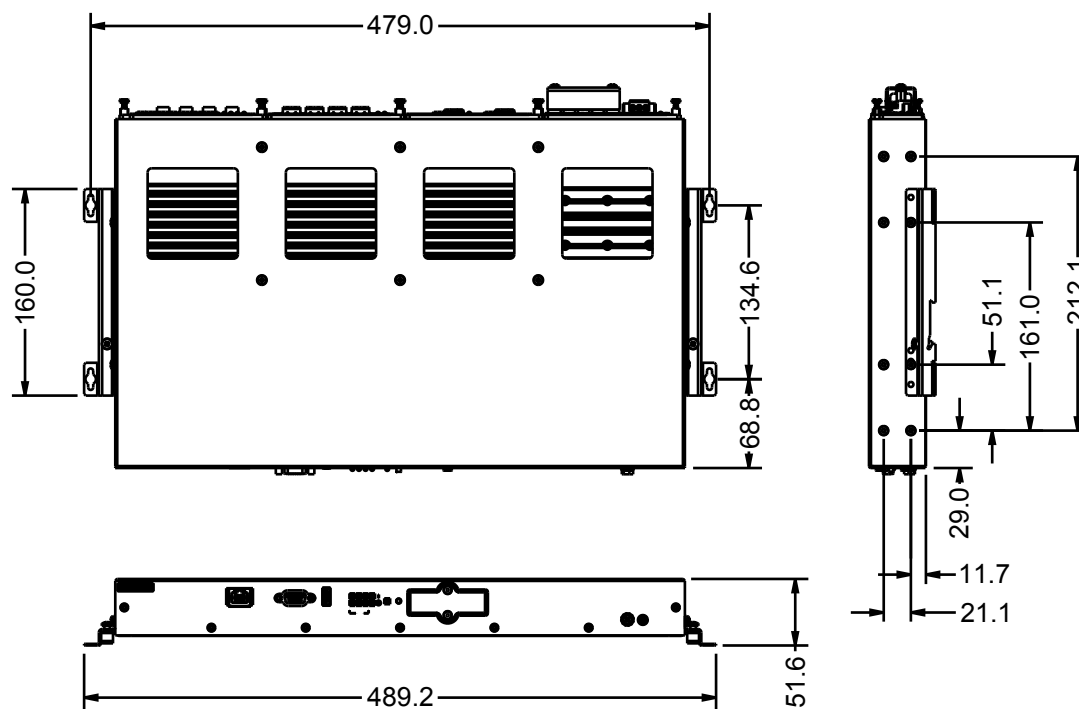
Figure 55: Panel and Din Rail Mount Dimensions
