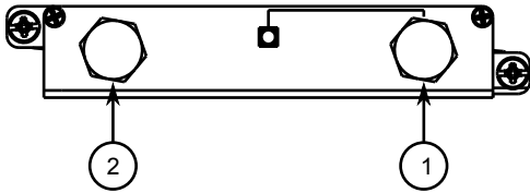
Figure 43: W11 and W21 Cellular Modems 1. Main Antenna SMA Connector 2. Receive Diversity Antenna SMA Connector
