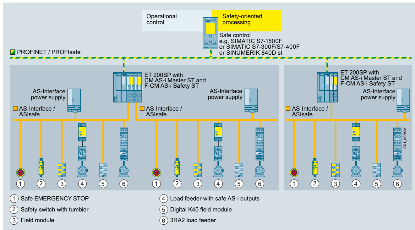
AS-Interface configuration consisting of an ET 200SP station with CM AS-i Master ST and F-CM AS-i Safety ST modules
