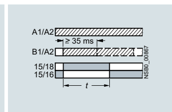
F 7PV1508-1A Pulse-forming with control signal (pulse generation at the output does not depend on duration of energizing)
