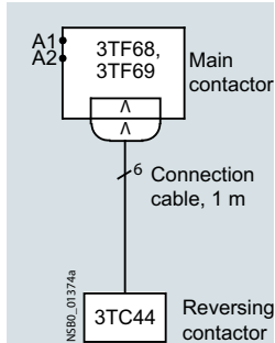
Circuit diagram for AC operation, 50/60 Hz, for AC control subject to strong interference
