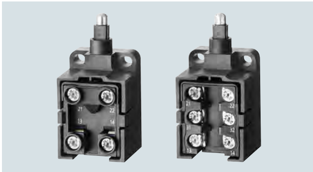
Open-type design
