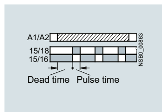
- 7PV1558 Clock-pulse, starting with interval (dead time, pulse time, and time setting ranges each separately adjustable)
