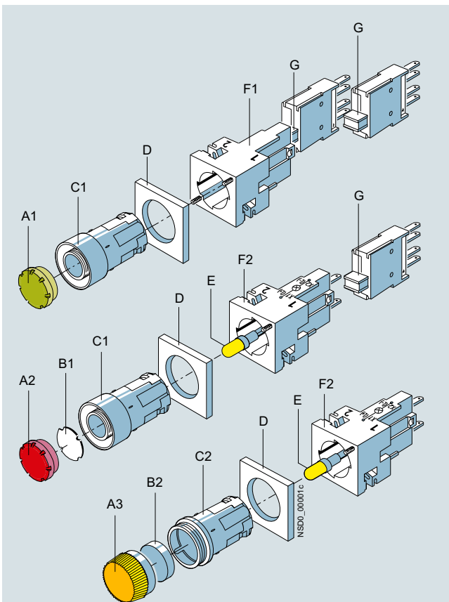
3SB2 pushbuttons with solder pins
