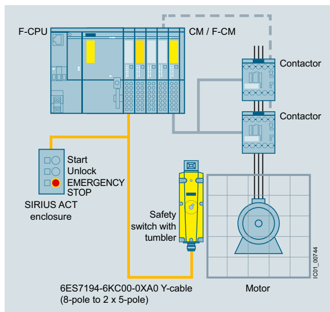
Connection to fail-safe control equipment via CM AS-i Safety ST and F-CM AS-i Safety ST
