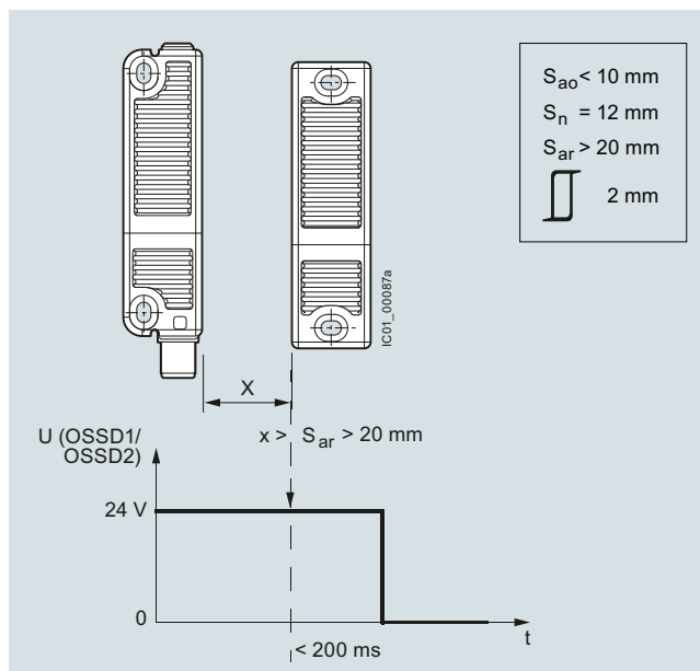
Switching interval: Output signal with OFF delay
