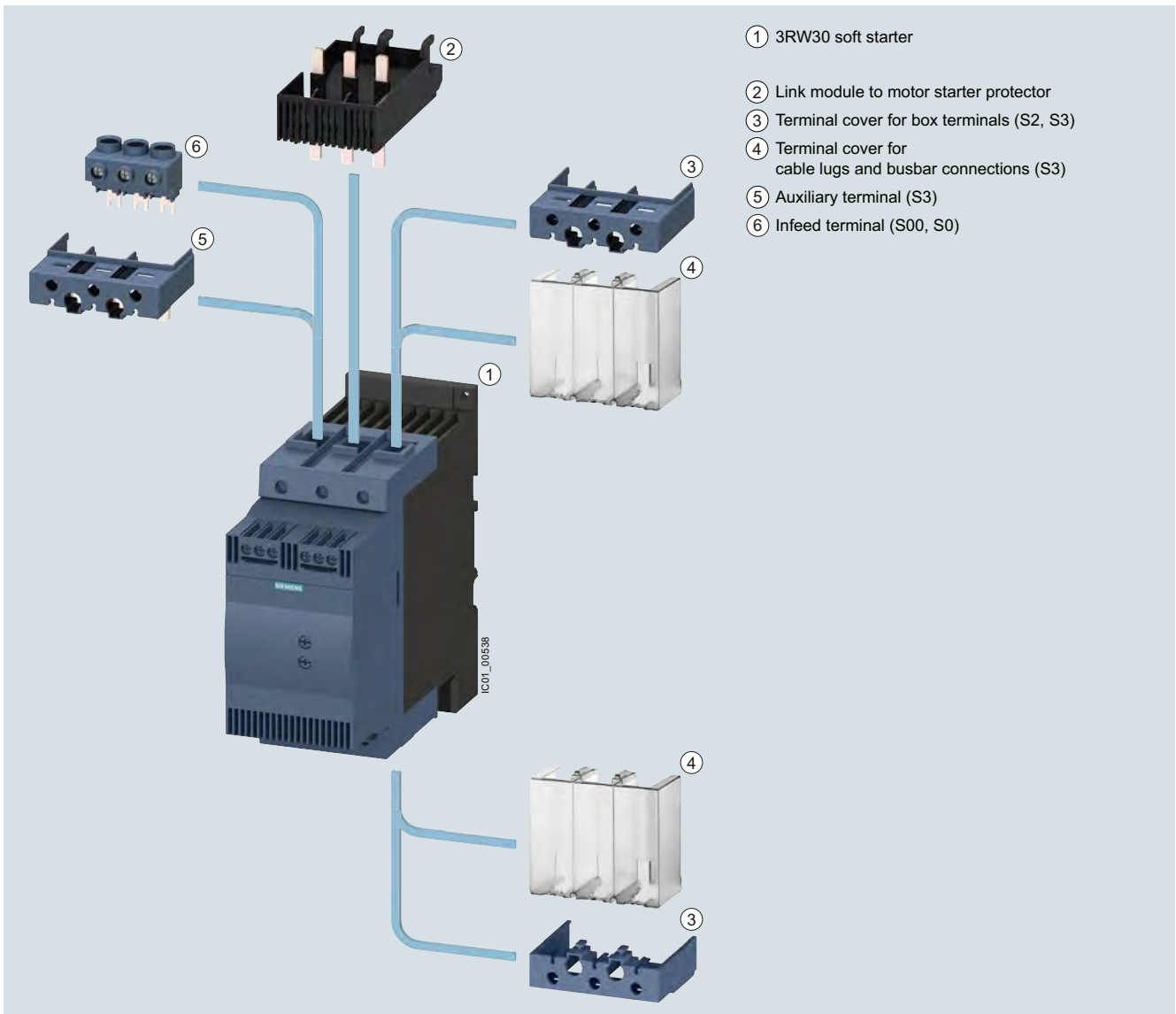
SIRIUS 3RW30 Basic Performance soft starter with accessories (see page 6/105)
