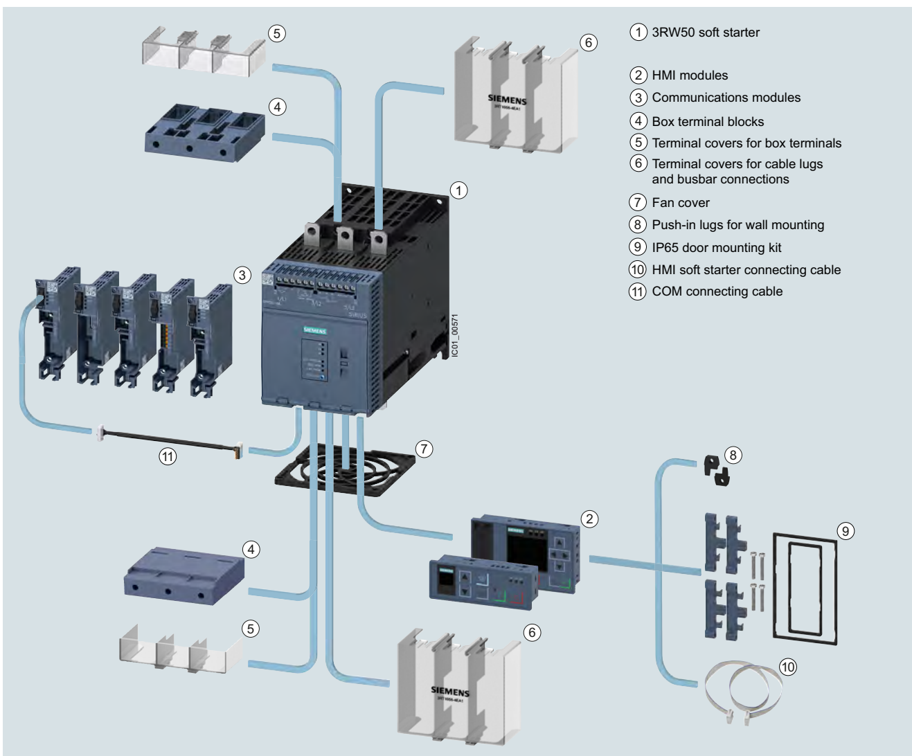
SIRIUS 3RW50 Basic Performance soft starter with accessories (see page 6/82), for expansion with HMI module or communications module
